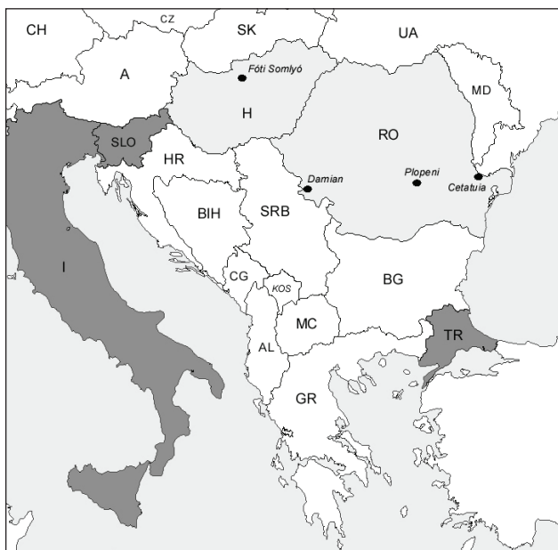
Fig. 3. Distribution of C. tergestinus in Europe: countries in dark grey – known occurrence; countries in light grey – new data.
